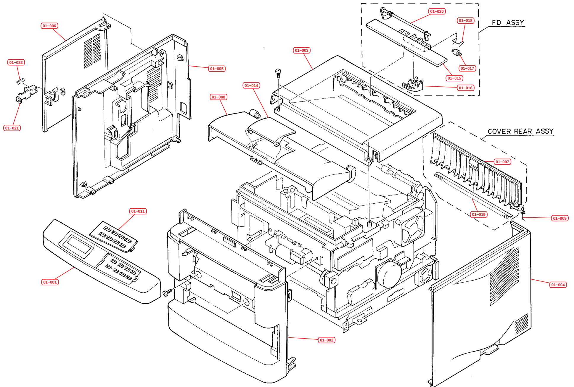
Fig.1 – Covers
