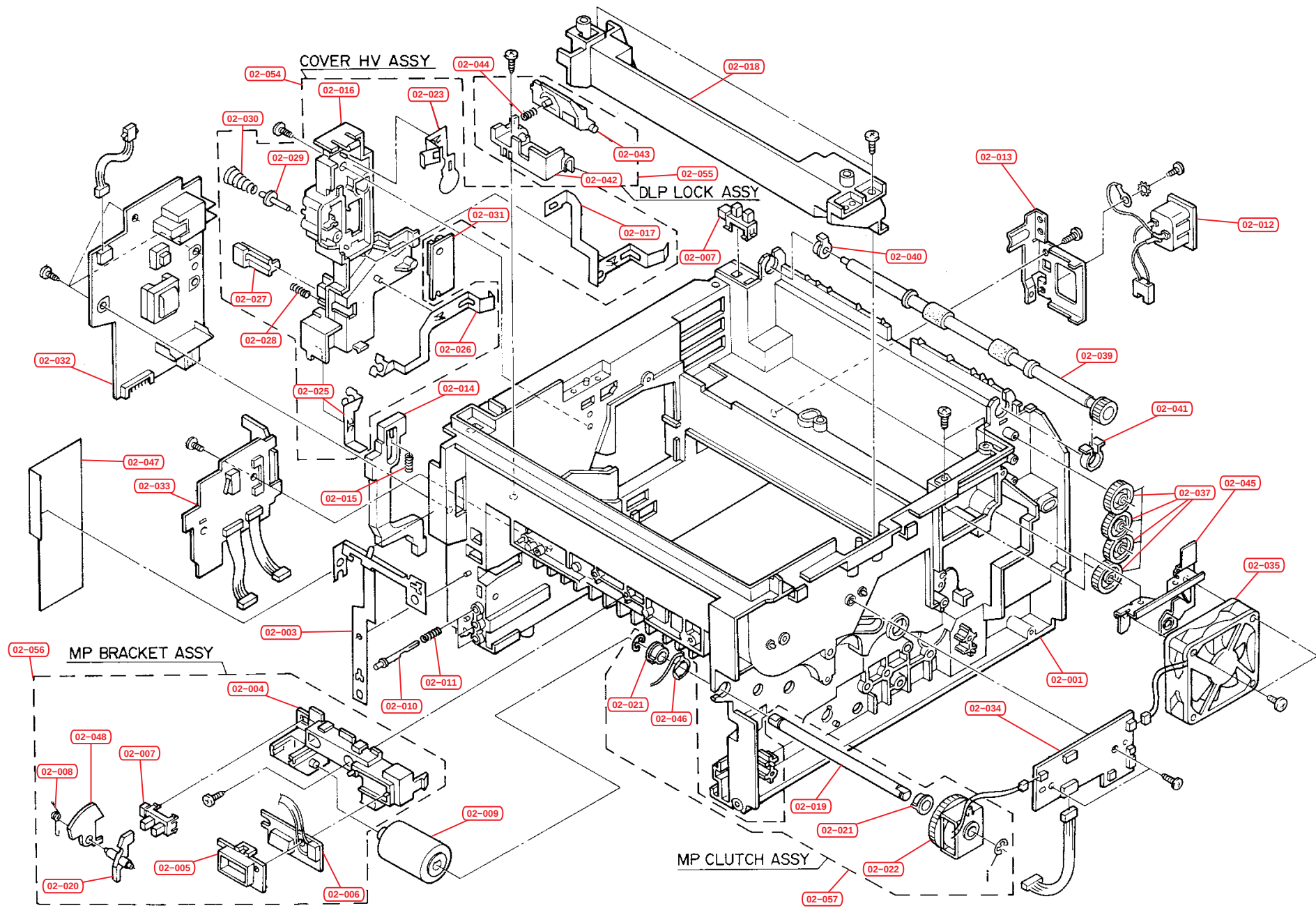
Fig.2 – Frame Unit
