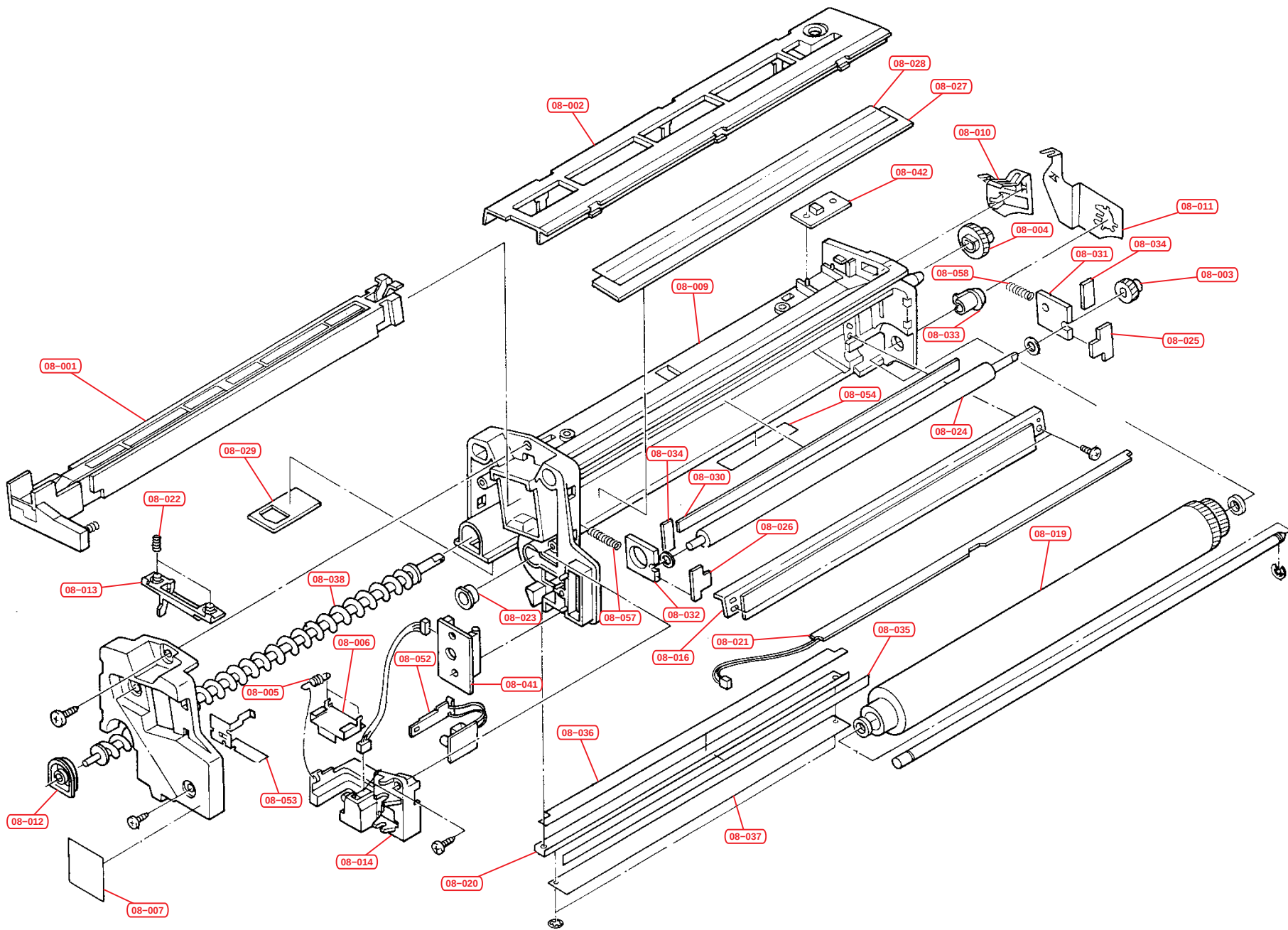
Fig.8 – Drum Unit
