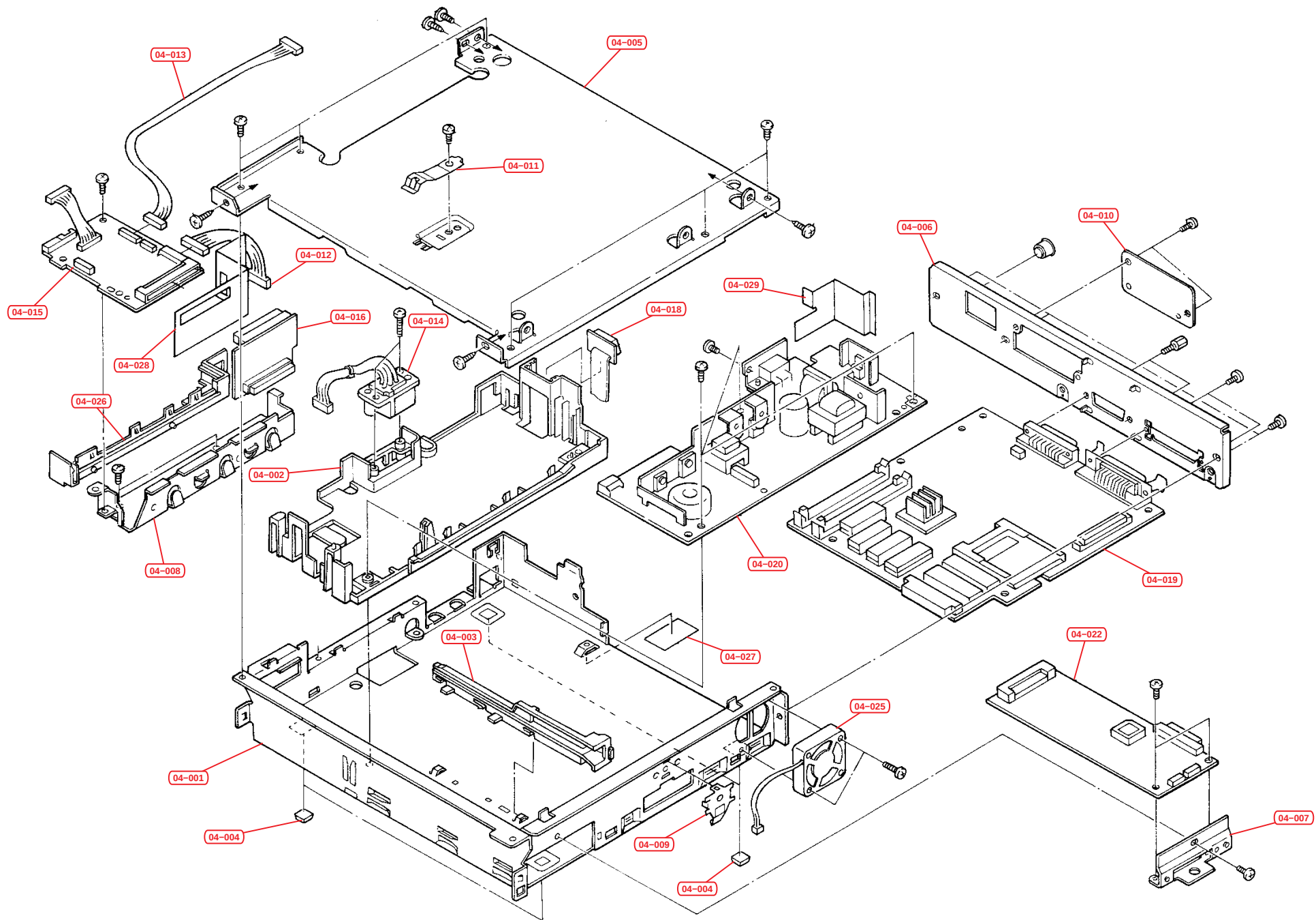
Fig.4 – Controller Unit
